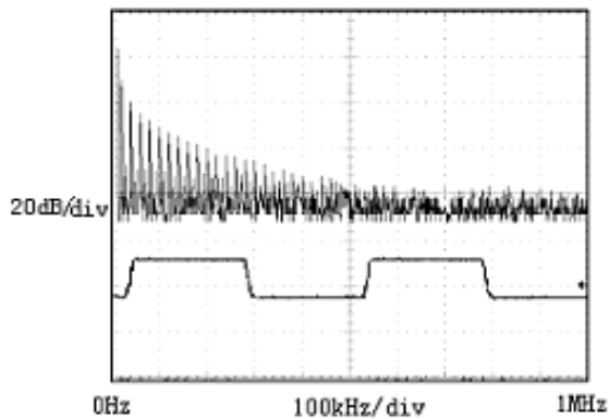
Figure 7. Driver Output Waveform and FFT Plot of YZ3085E Transmitting a 20kHz Signal
