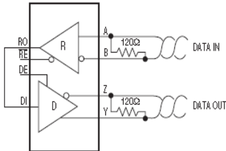
Figure 8. Line Repeater for YZ3085E
