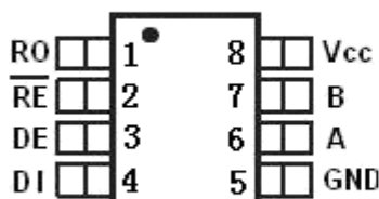
YZ3085E Pin figure
