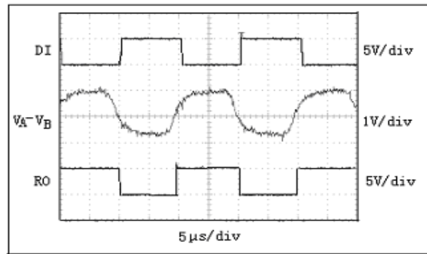
Figure 9. YZ3085E System Differential Voltage at 50kHz Driving 4000ft of Cable
