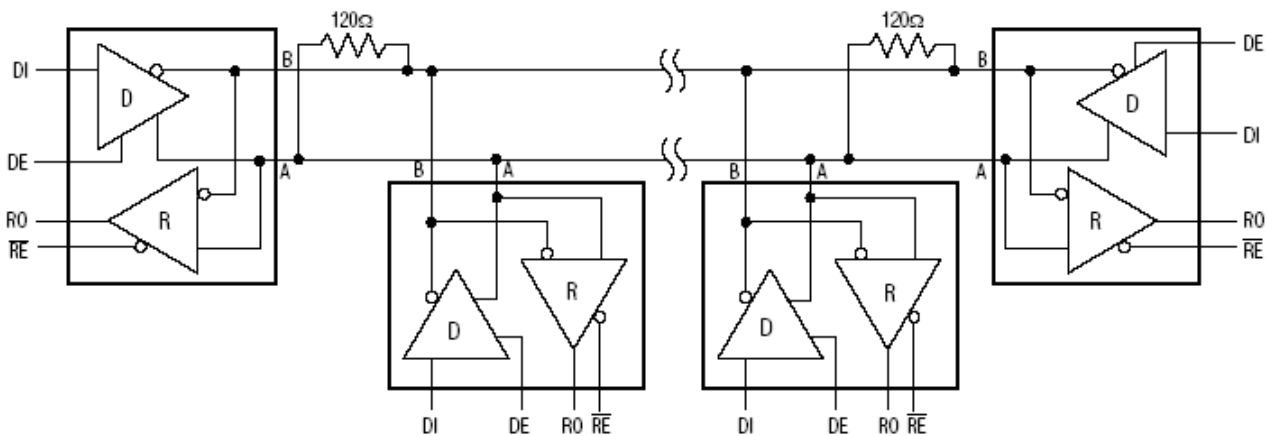
Figure 10. YZ3085E Pin Configuration and Typical Half-Duplex Operating Circuit
