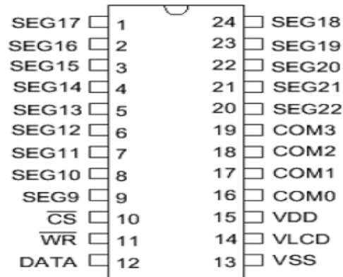
SOP24
